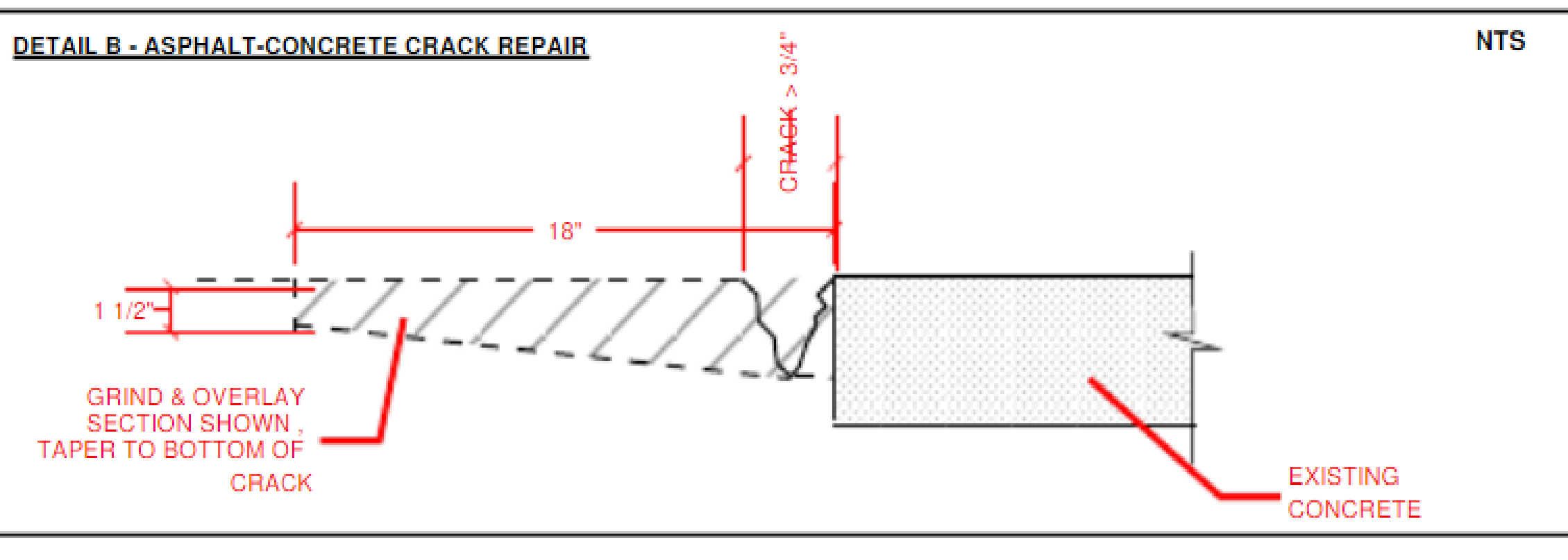
DETAIL B - ASPHALT-CONCRETE CRACK REPAIR
