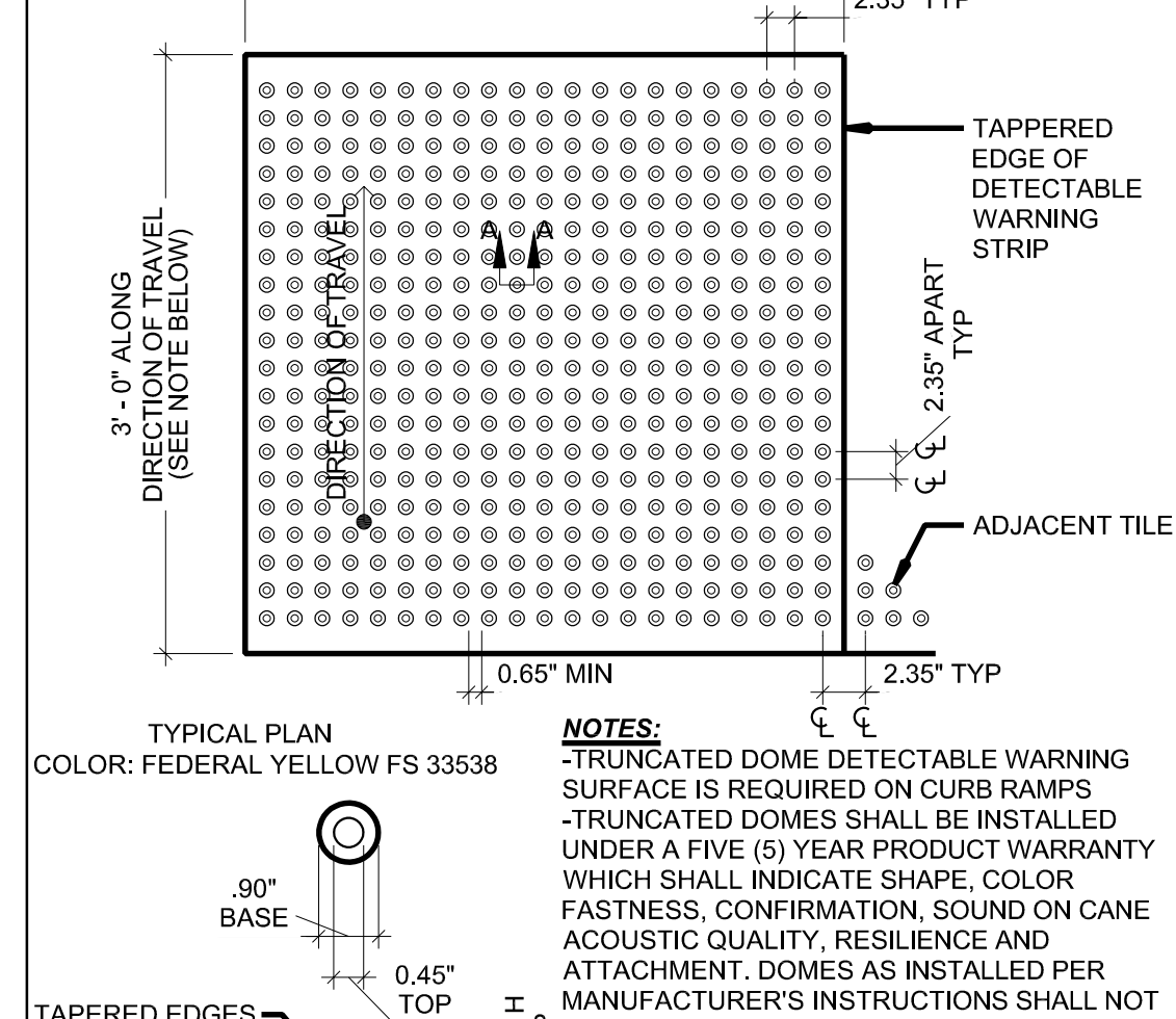
TRUNCATED DOMES DETAILS 1"=1'-0" 14
