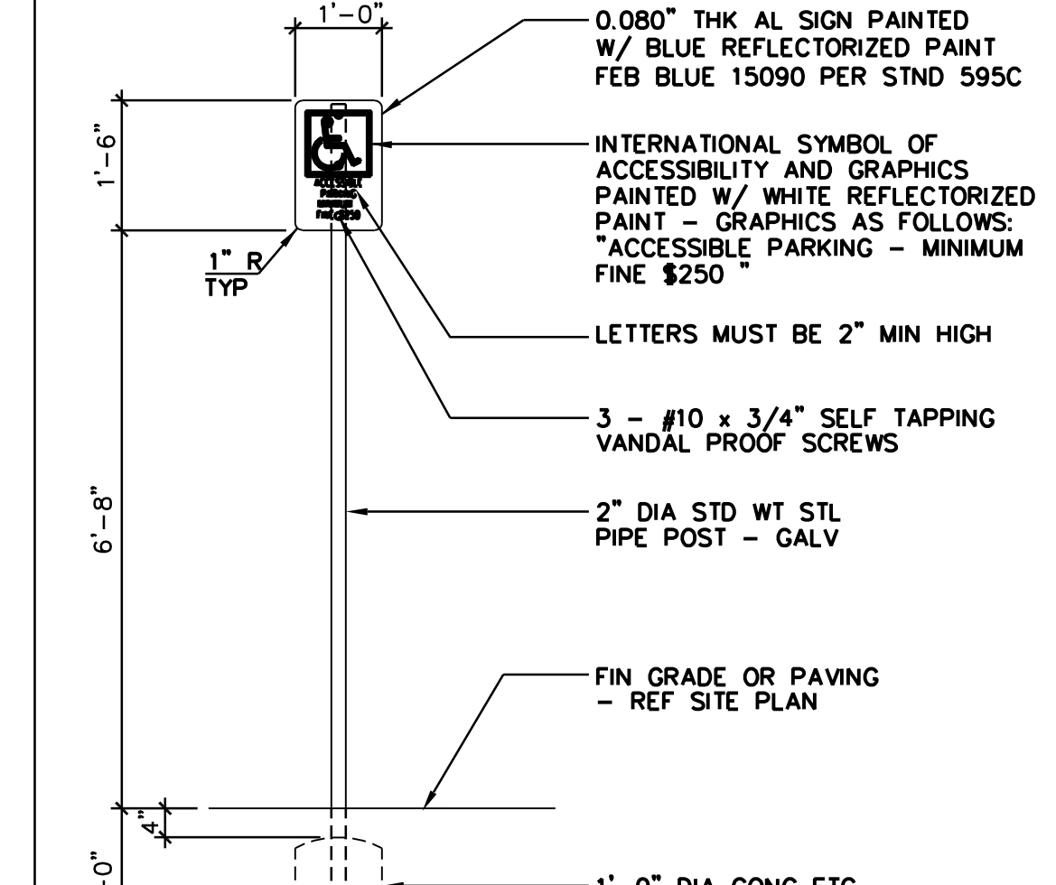
PARKING SIGN 1/2"=1'-0" 2
