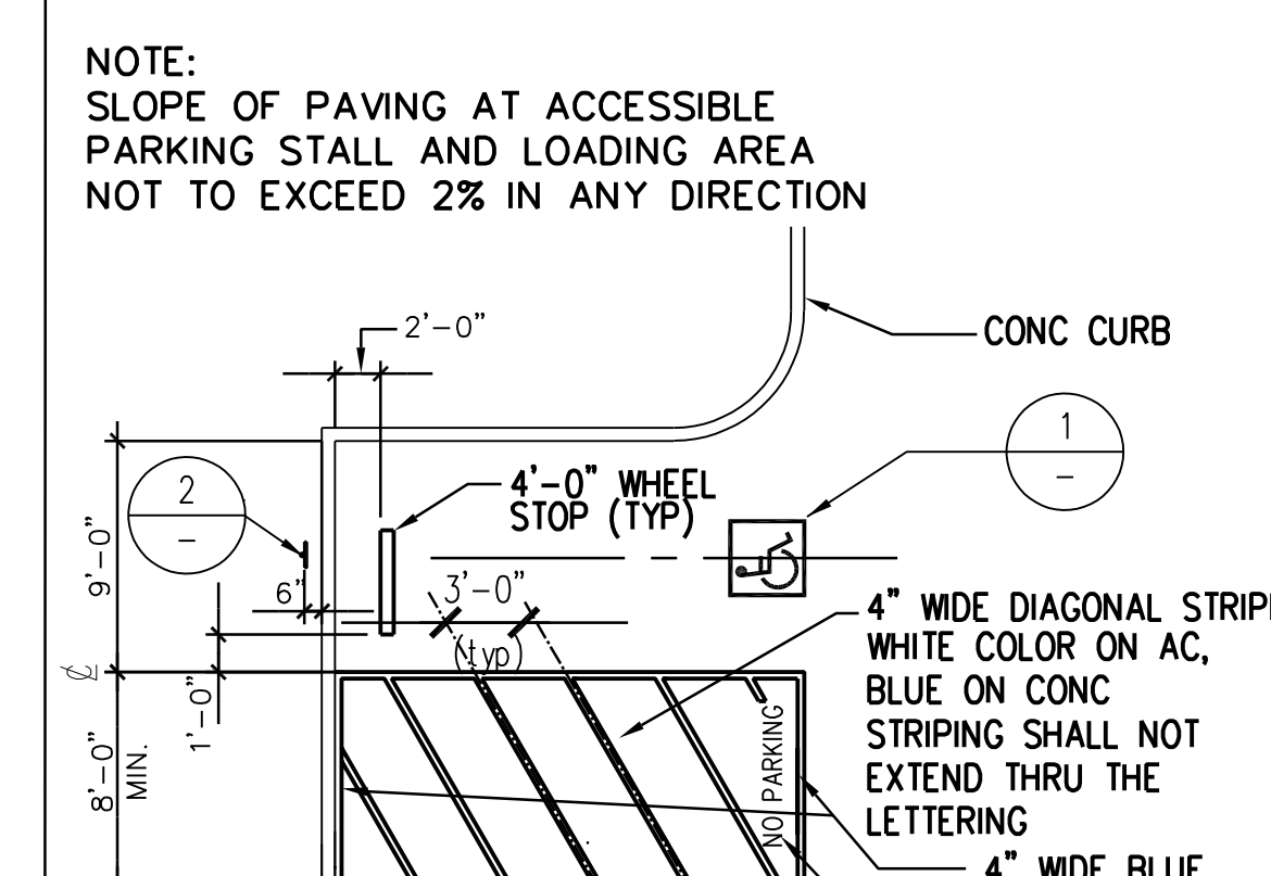
PERPENDICULAR PARKING 1/8"=1'-0" 11
