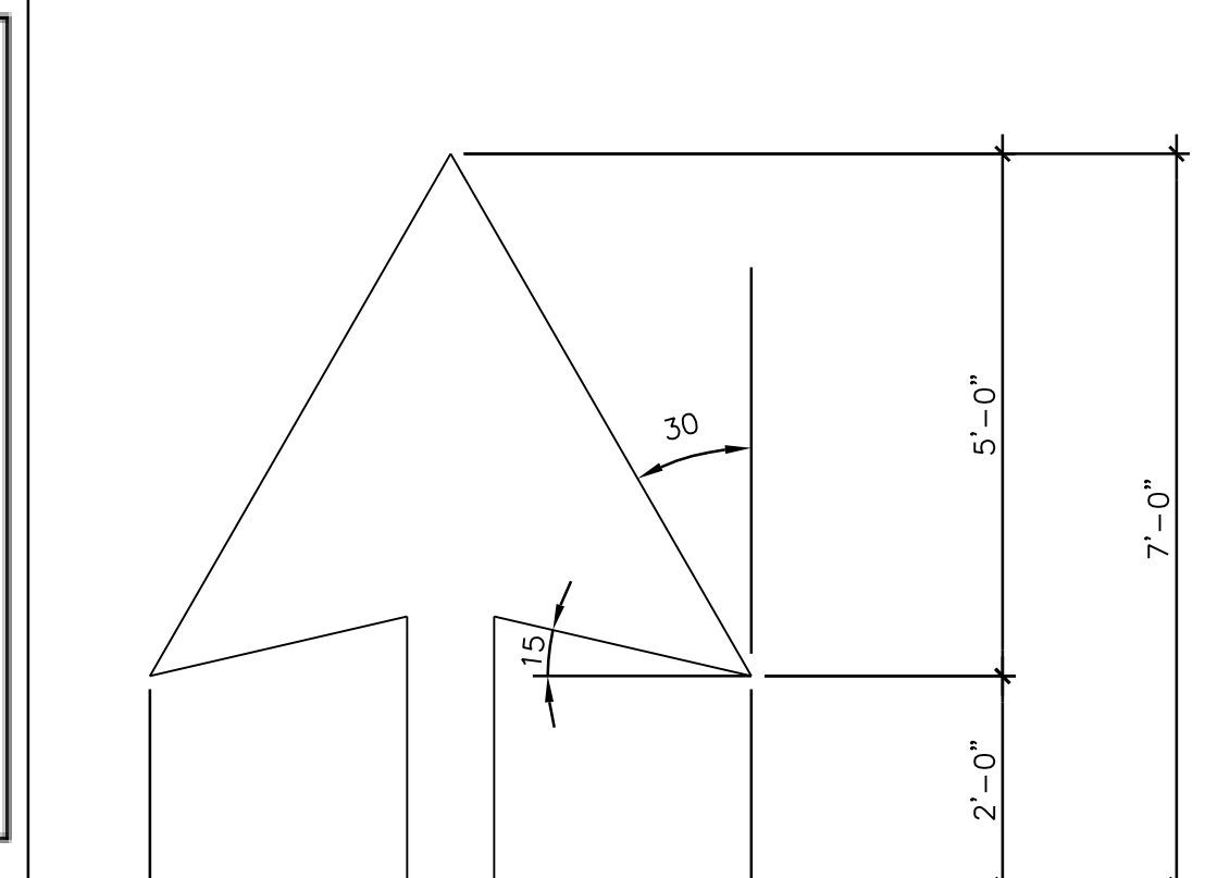
TRAFFIC ARROW 1/2"=1'-0" 15
