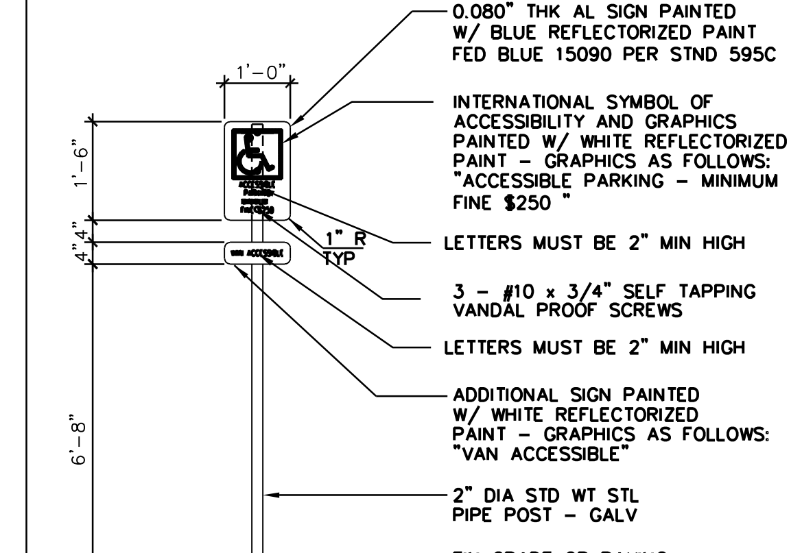
VAN ACCESS. PARKING SIGN 1/2"=1'-0" 3
