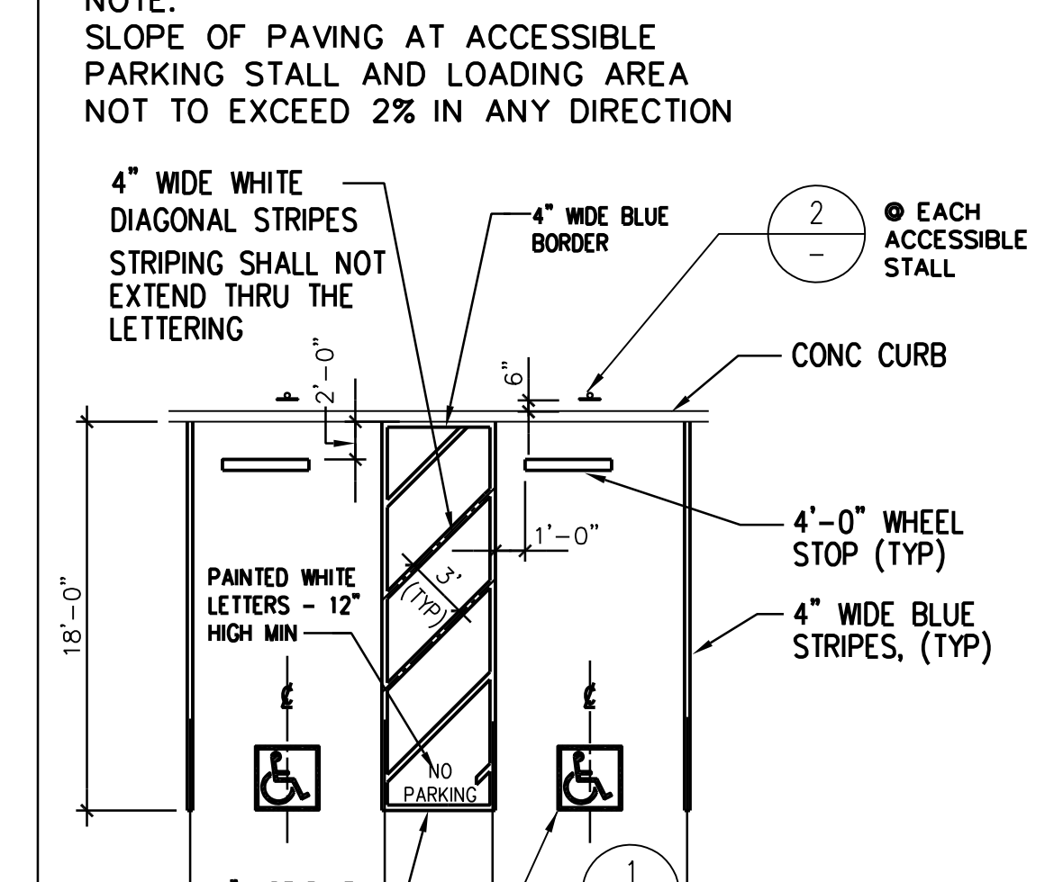
ACCESSIBLE STALL STRIPING DETAIL 1/8"=1'-0" 10
