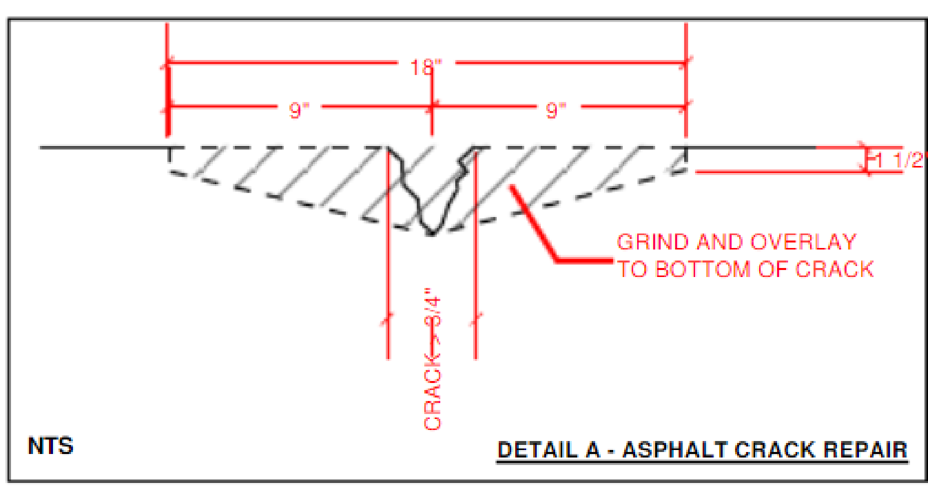
DETAIL A - ASPHALT CRACK REPAIR
