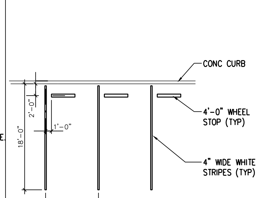
STANDARD STALL STRIPING DETAIL 1/8"=1'-0" 7
