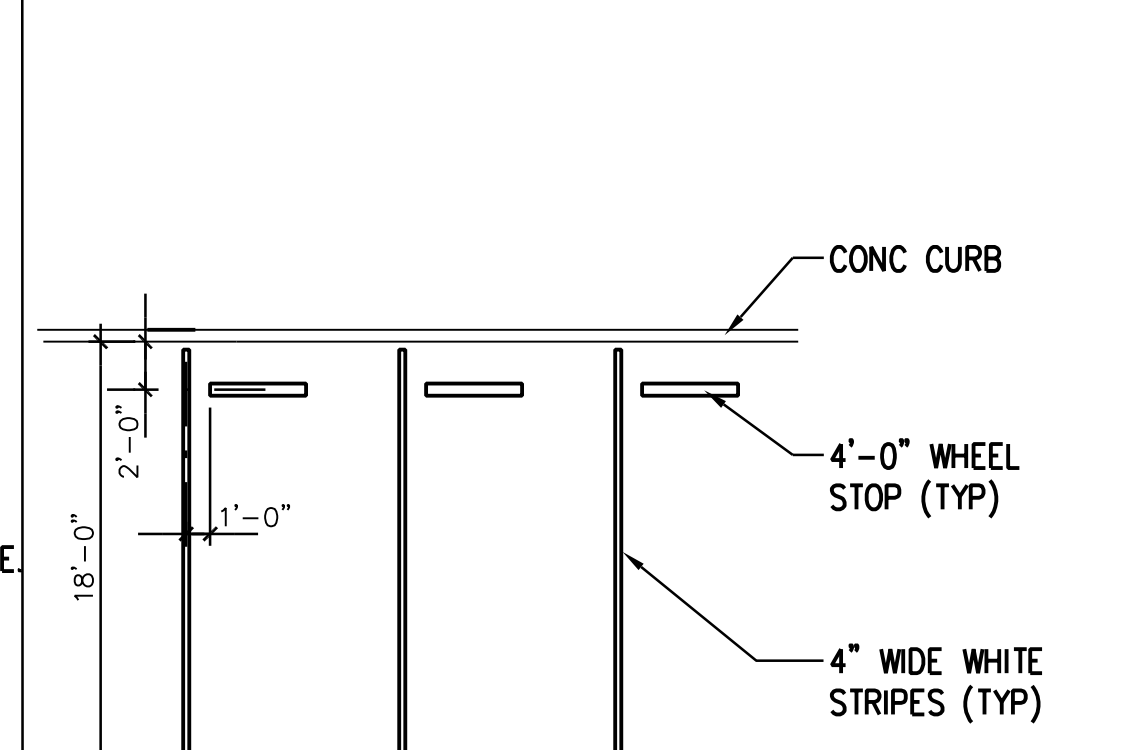
STANDARD STALL STRIPING DETAIL 1/8"=1'-0" 7
