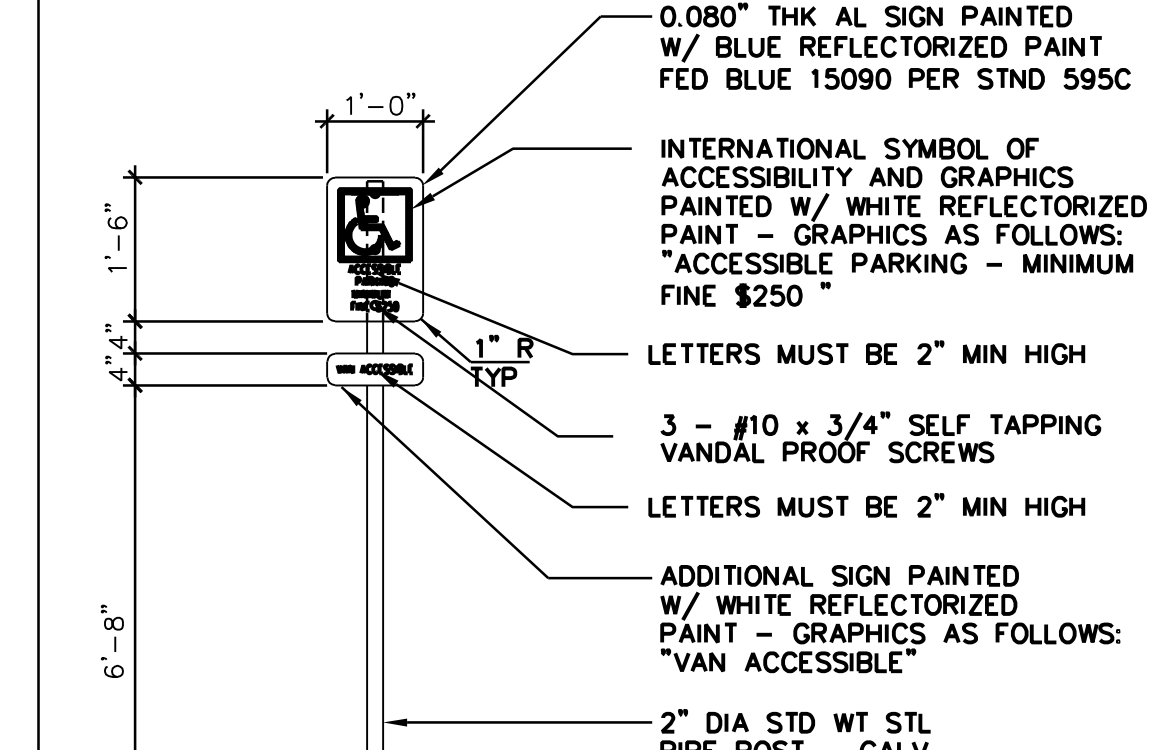
VAN ACCESS. PARKING SIGN 1/2"=1'-0" 3
