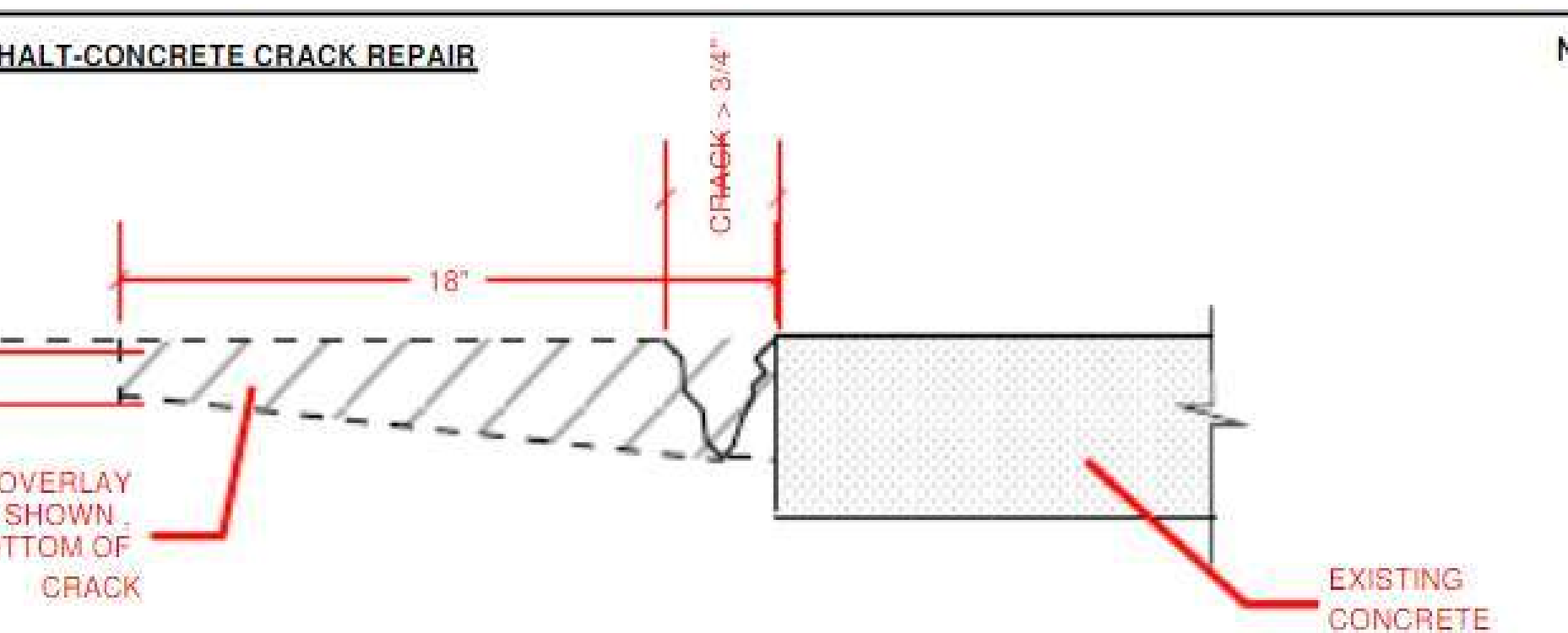
DETAIL B - ASPHALT-CONCRETE CRACK REPAIR
