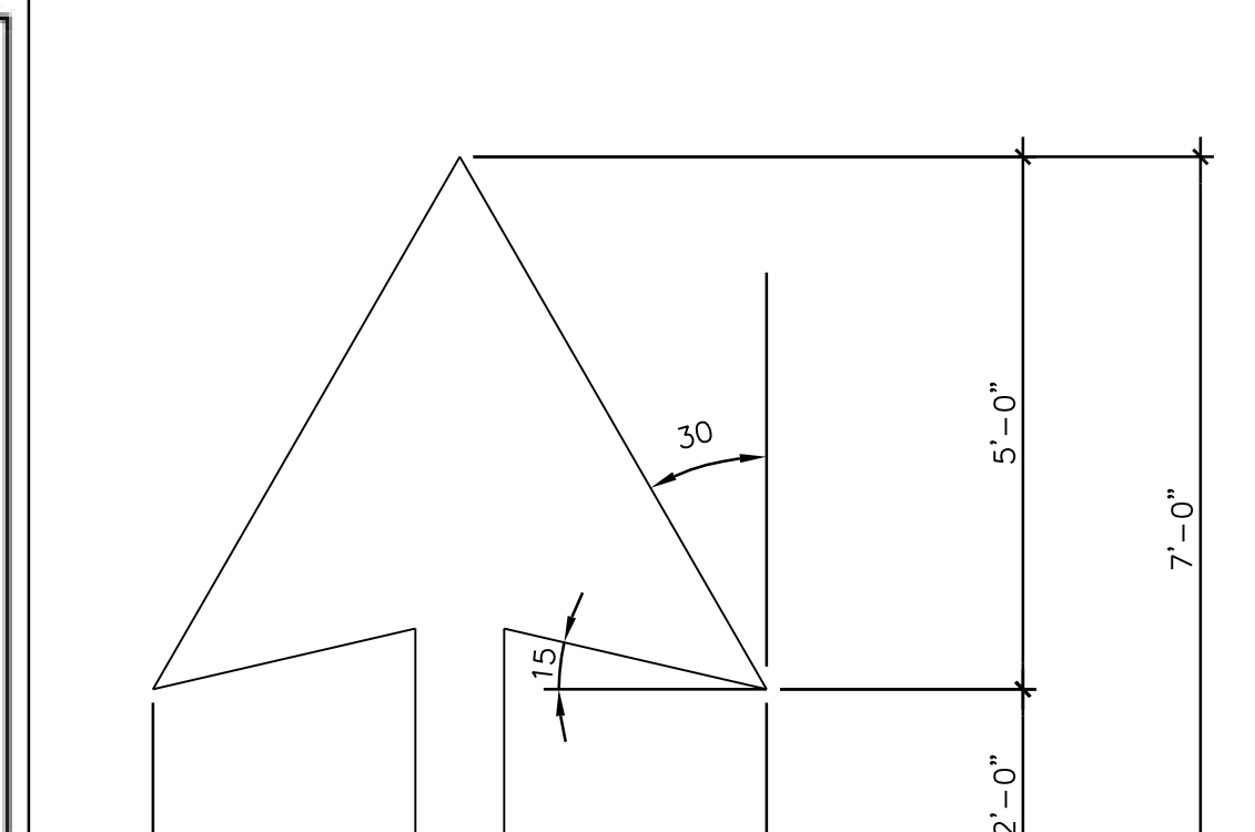
TRAFFIC ARROW 1/2"=1'-0" 15
