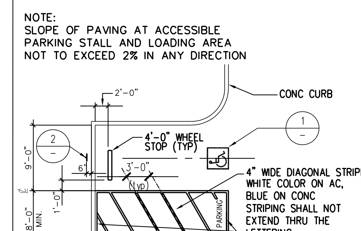
PERPENDICULAR PARKING 1/8"=1'-0" 11
